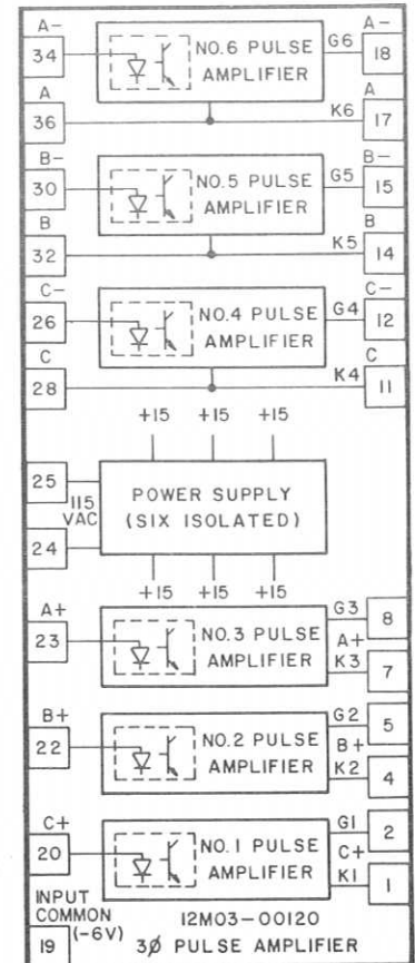
FIGURE 1 SIMPLIFIED SCHEMATIC
